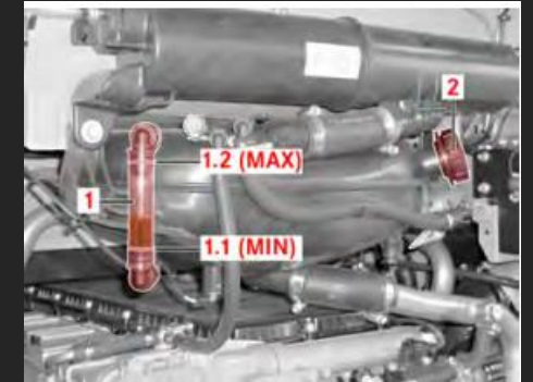
Coolant Sight-glass
